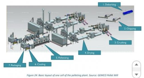
Figure 24: Basic layout of one cell of the pelleting plant. Source: GEMCO Pellet Mill
